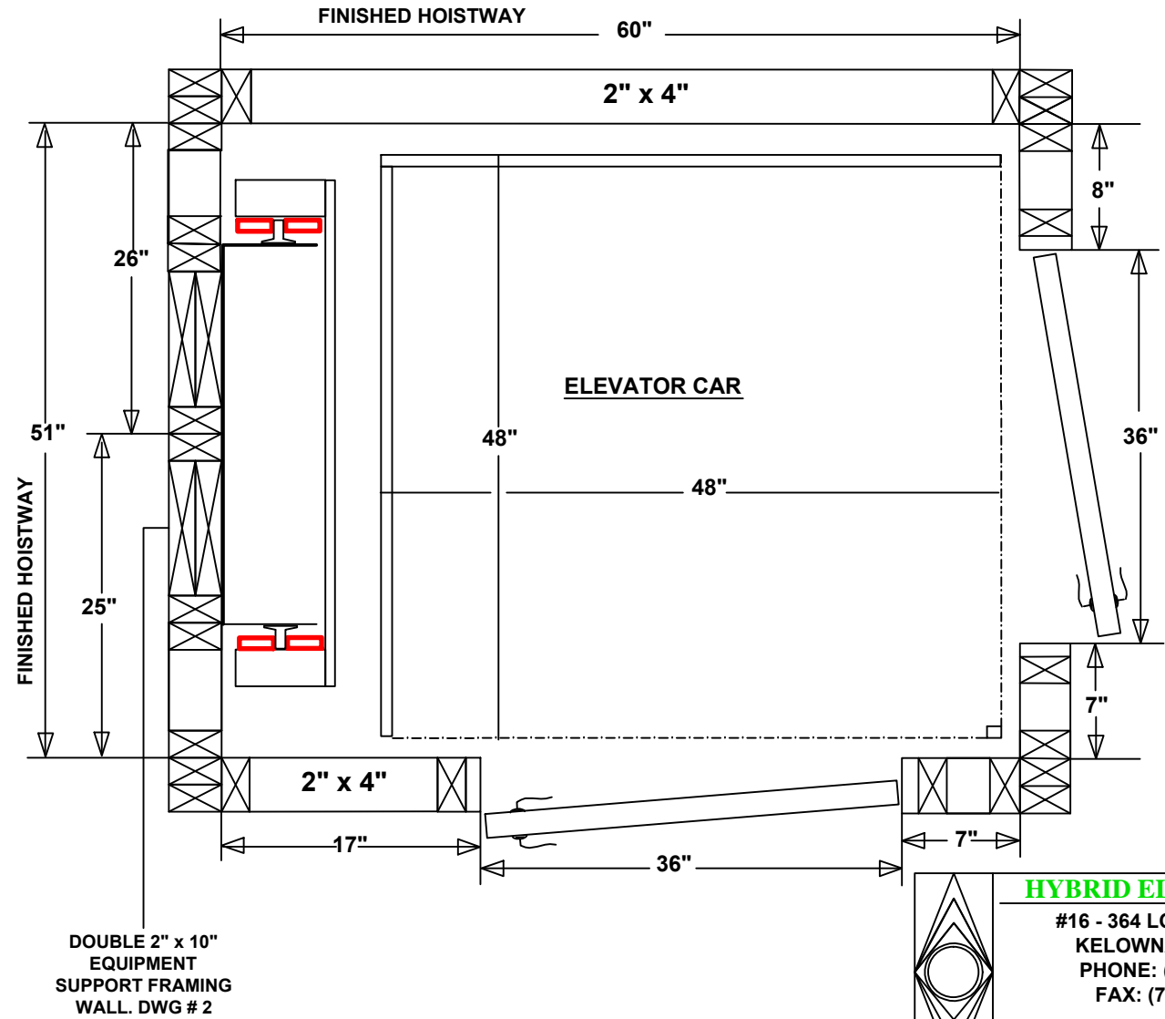
TYPE # 3 LEFT HAND DRIVE WALL 4' x 4' CAR
