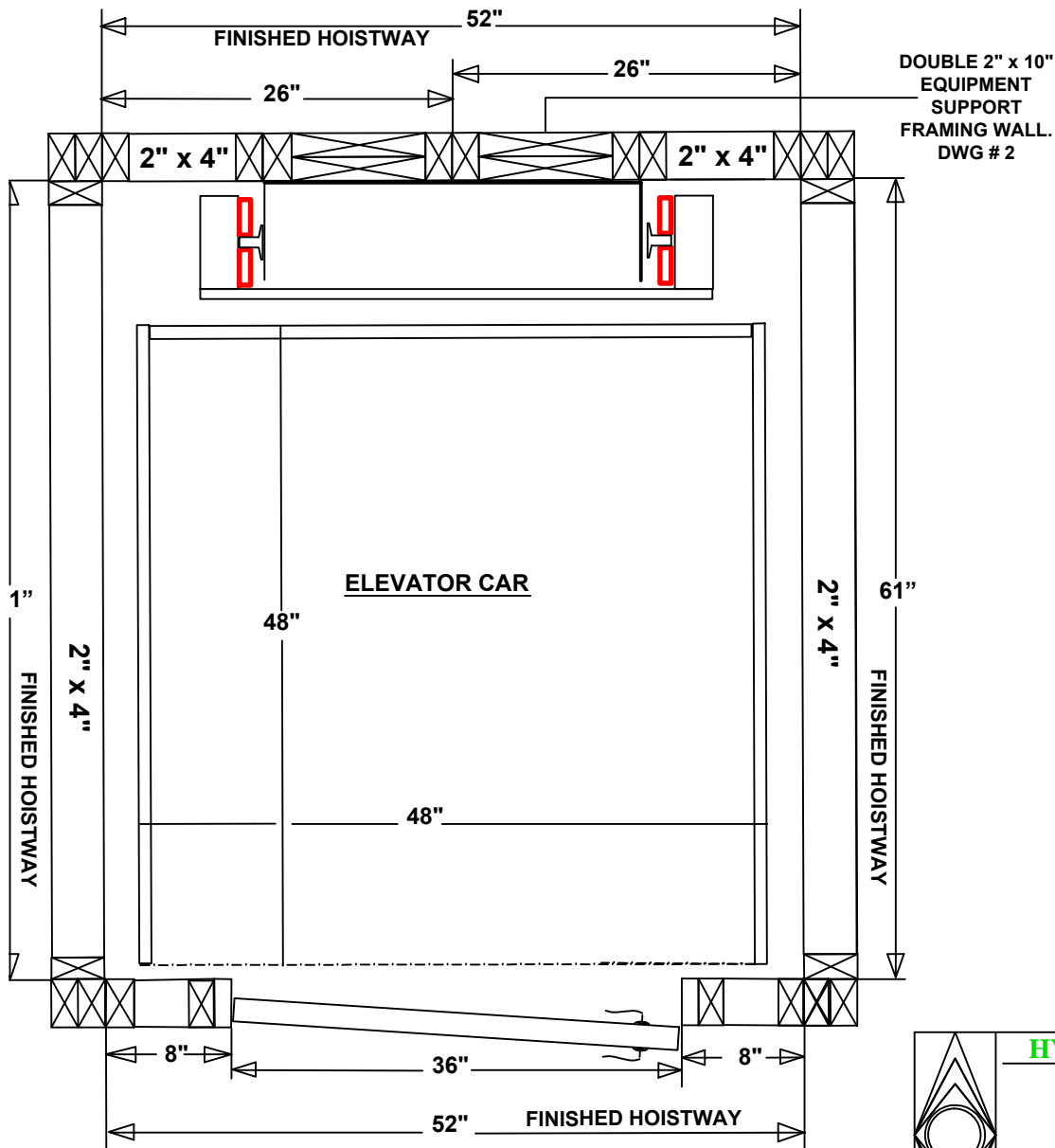
TYPE # 1 REAR DRIVE WALL 4' x 4' CAR
