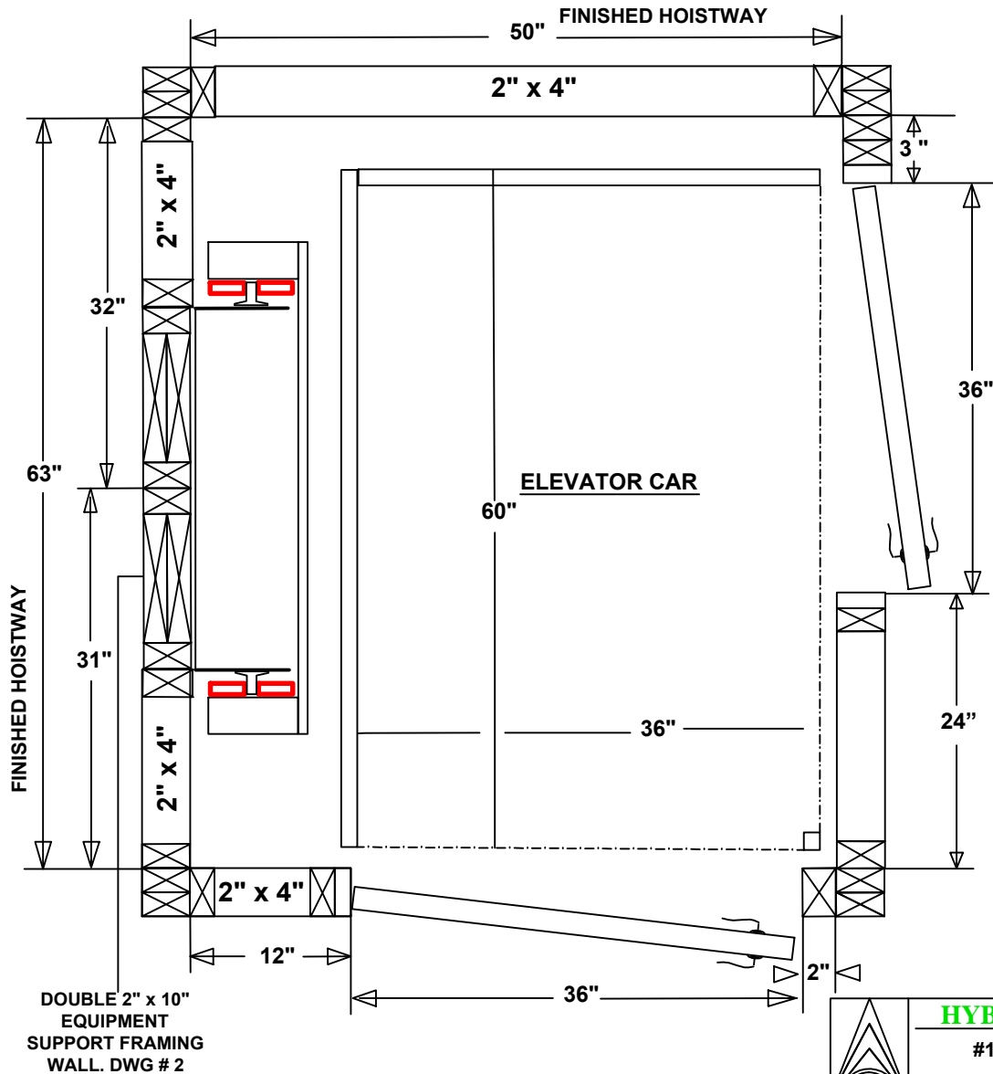
TYPE # 3 LEFT HAND DRIVE WALL 3' x 5' CAR
