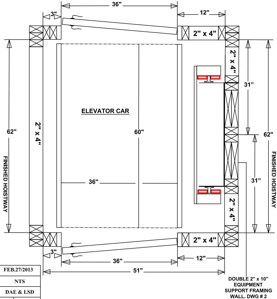
TYPE # 2 RIGHT HAND DRIVE WALL 3' x 5' CAR
