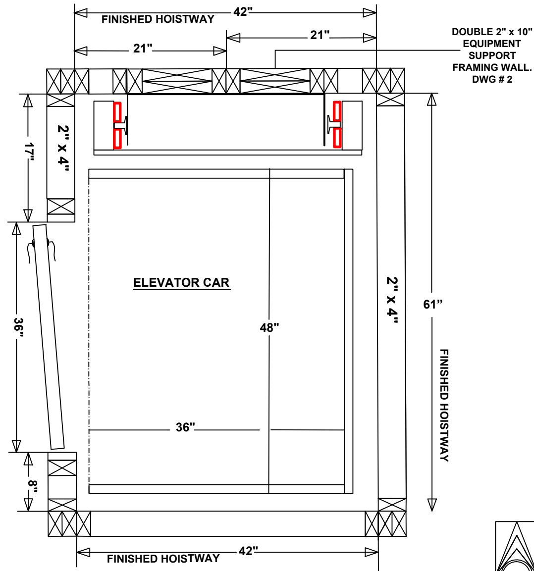
TYPE # 1 LEFT DRIVE WALL SIDE ENTRY 3' x 4' CAR
